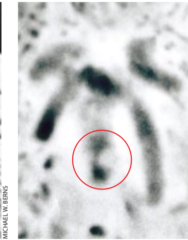
FEATS ACCOMPLISHED by laser scissors include etching of grooves ( left ) in the zona pellucida around a fertilized mouse egg ( inset ) to facilitate implantation. They also include removing a V-shaped wedge from a chromosome ( right ) in a living cell from a kangaroo rat. At its widest, the wedge is about one micron across.
